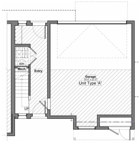
① Level 1 - Unit Type A - Furniture Plan 3/16" = 1'-0"
