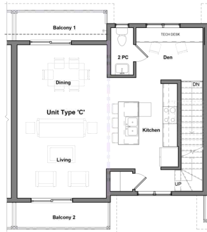
⑧ Level 2 - Unit Type C - Furniture Plan 3/16" = 1'-0"
