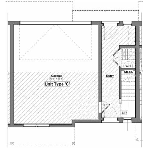
⑦ Level 1 - Unit Type C - Furniture Plan 3/16" = 1'-0"
