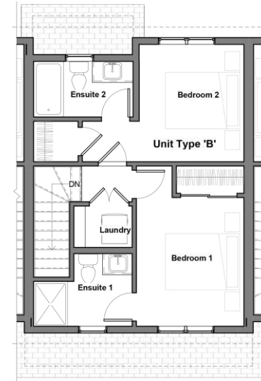
⑥ Level 3 - Unit Type B - Furniture Plan 3/16" = 1'-0"
