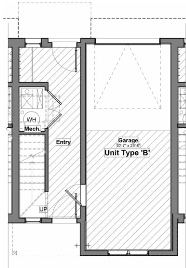
④ Level 1 - Unit Type B - Furniture Plan 3/16" = 1'-0"
