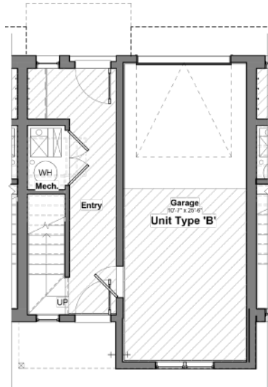
4 Level 1 - Unit Type B - Furniture Plan 3/16" = 1'-0"
