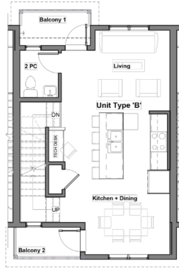
5 Level 2 - Unit Type B - Furniture Plan 3/16" = 1'-0"
