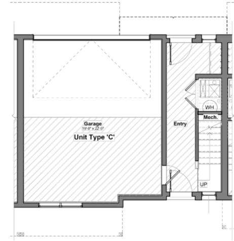
7 Level 1 - Unit Type C - Furniture Plan 3/16" = 1'-0"
