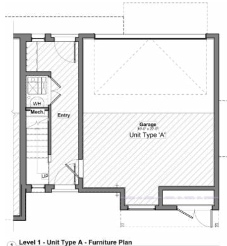
① Level 1 - Unit Type A - Furniture Plan 3/16" = 1'-0"
