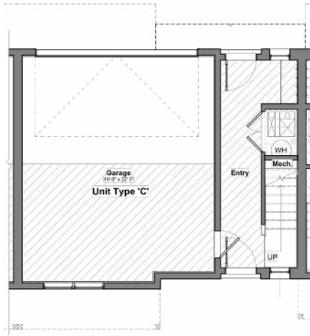
7 Level 1 - Unit Type C - Furniture Plan 3/16" = 1'-0"
